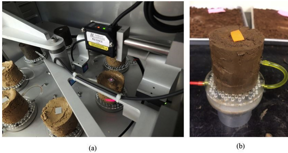
Fig. 4. (a) Inside of TypoSoil™ Device (TypoSoil™ User Manual), (b) Standard soil core ( \phi = 5 \text{ cm} , h = 5 \text{ cm} - 100 \text{ cm}^3 ).
